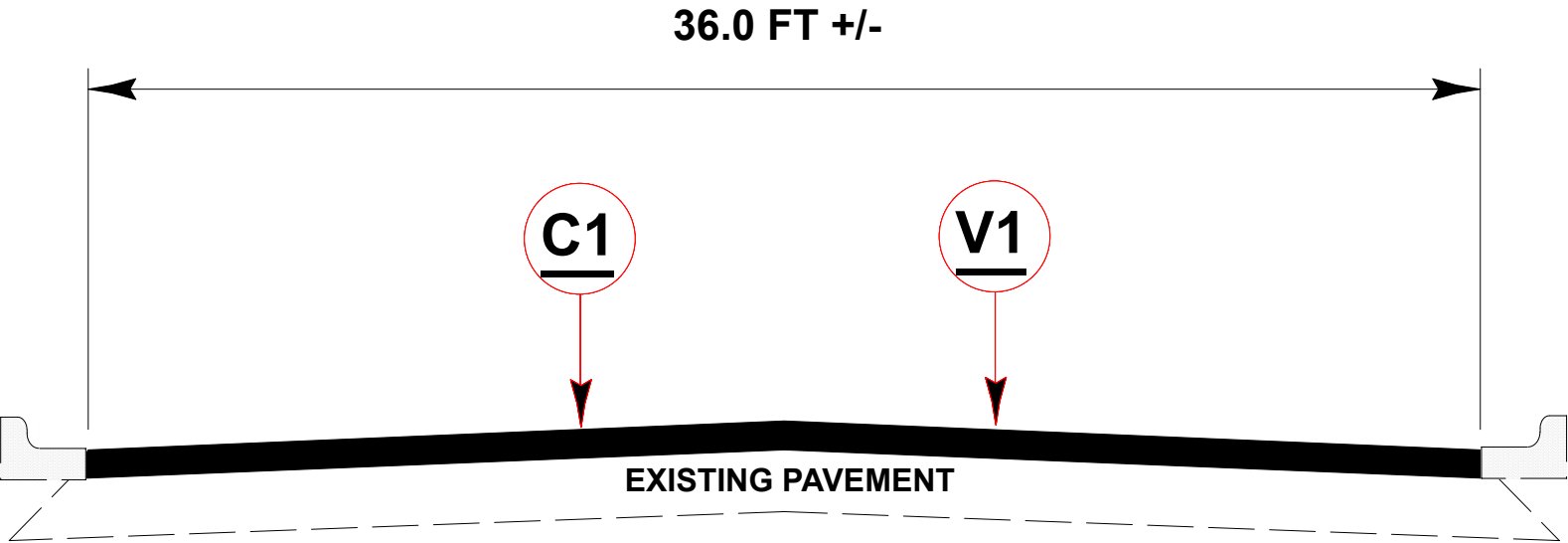
TYPICAL SECTION # 2 MAP(S) # 3
