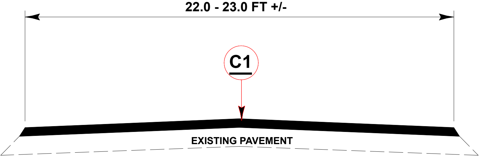
TYPICAL SECTION # 1 MAP(S) # 1, 2, & 4
