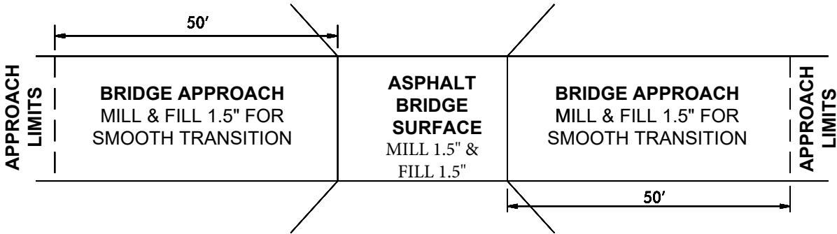
DETAIL FOR MAP #1,2, & 6 / STRUCTURE #0022, 0096, & 0086
